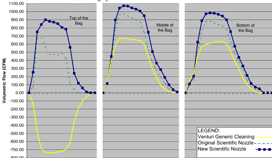
Figure1: Volumetric Flow throughout the Entire Bag for all systems at 100psig
